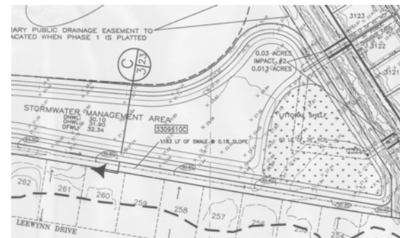
◀ Partial image of Approved As-Built Plans for Villages at Pine Tree from Step 6.
