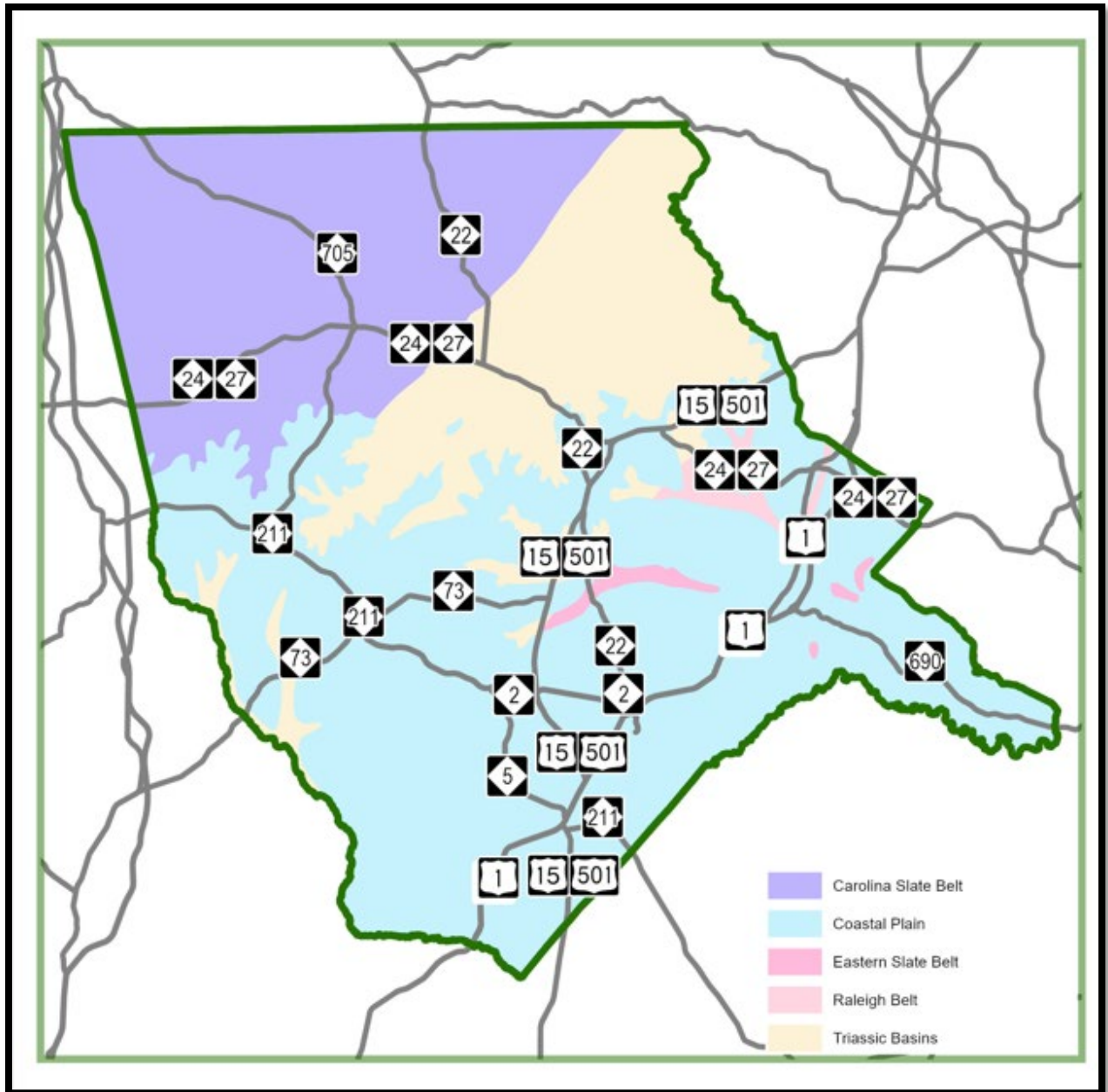
Figure 6.1 Geology of Moore County, Source: Land Use Plan Data 2013
