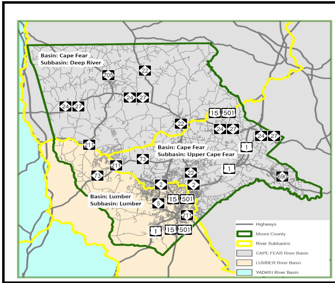
Figure 6.3: Moore County River Basins: (Source: Moore County GIS)
