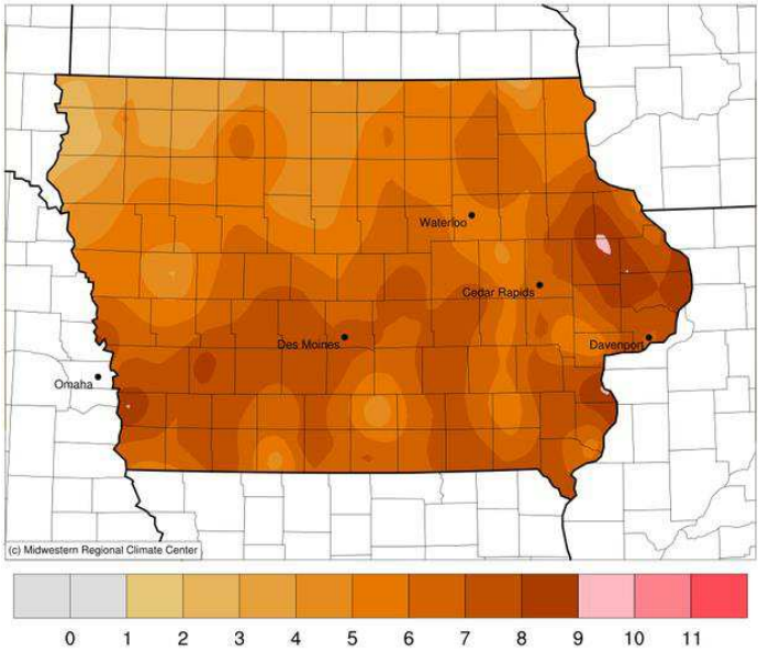
Average Temperature (°F): Departure from 1981-2010 Normals October 17, 2016 to October 23, 2016
