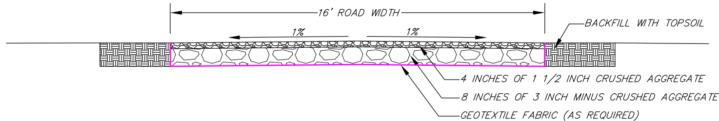
TYPICAL ROAD CROSS SECTION
