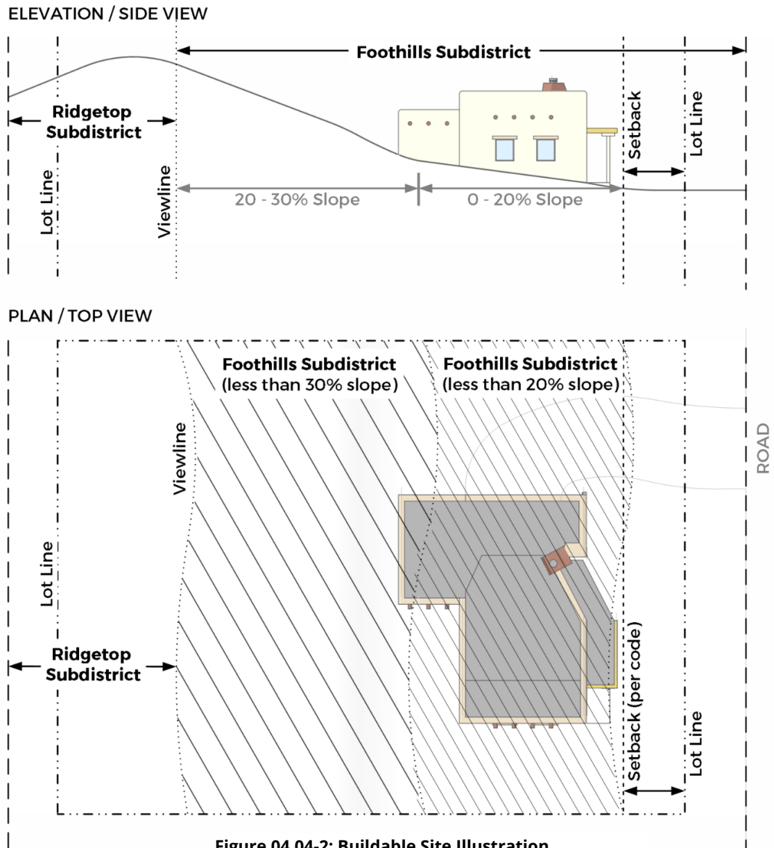
Figure 04.04-2: Buildable Site Illustration
