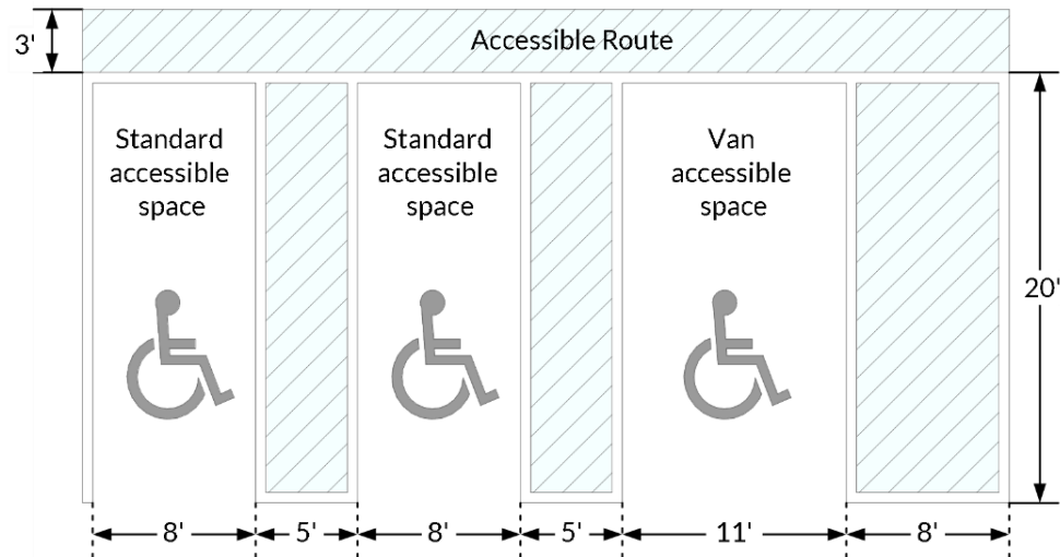
Figure 07.07-2: Accessible Space and Access Design
