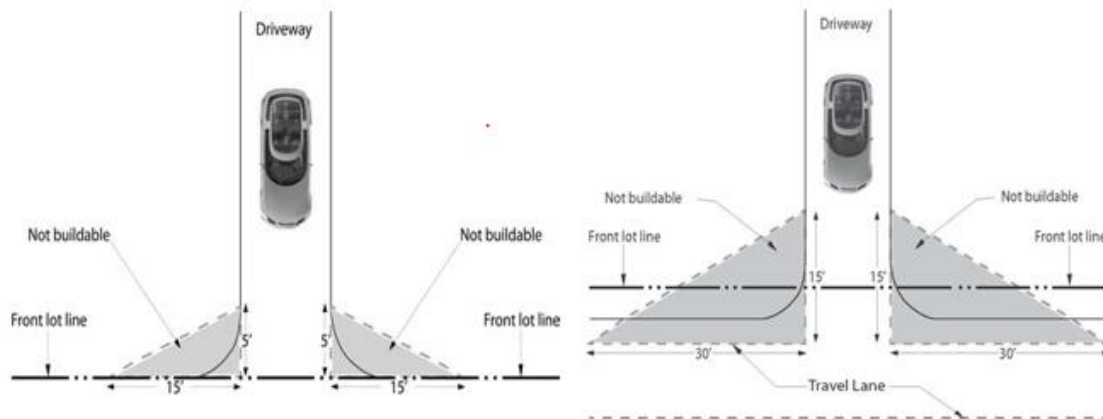
Figure 03.05-1: Visibility at Driveway Intersections
