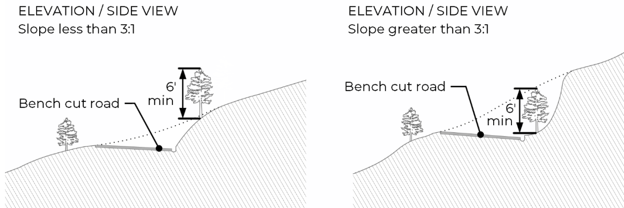
Figure 04.04-5: Planting on Slopes
