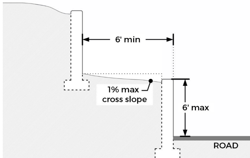
Figure 04.04-7: Retaining Wall Requirements
