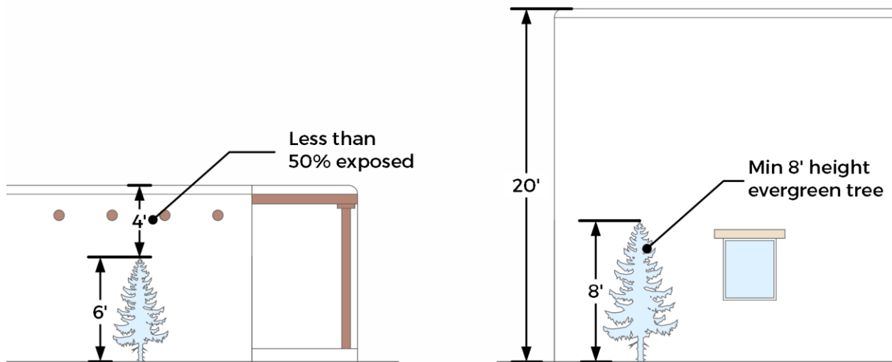
Figure 04.04-6: Landscaping Coverage of Structure
