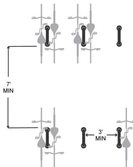
Figure 07.07-7: Bicycle Rack Spacing Requirements
