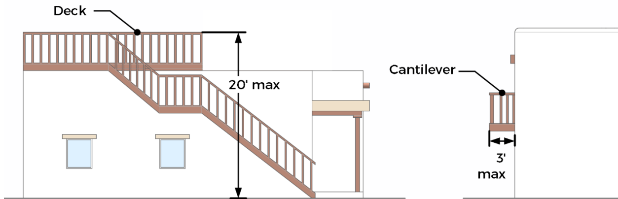
Figure 04.04-4: Height and Depth for Cantilevers
