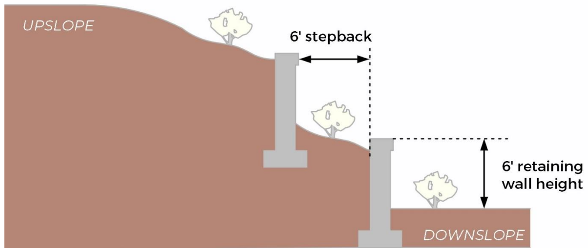
Figure 07.06-1: Retaining Wall Terracing
