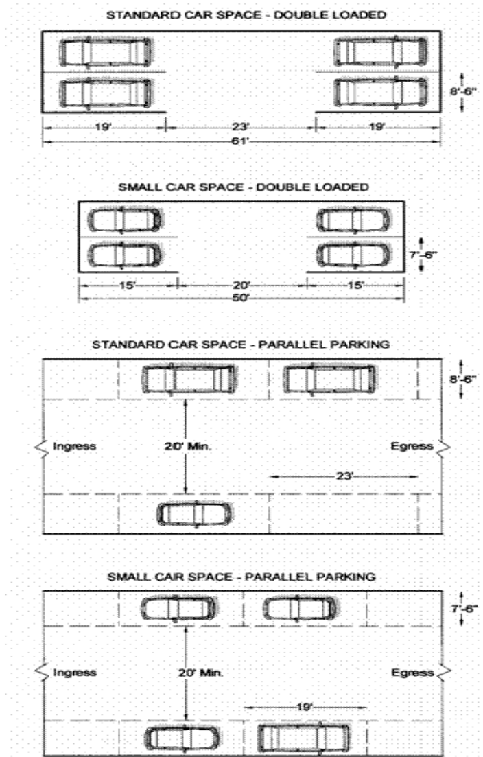
Figure 07.07-3: Non-Angle Parking Requirements
