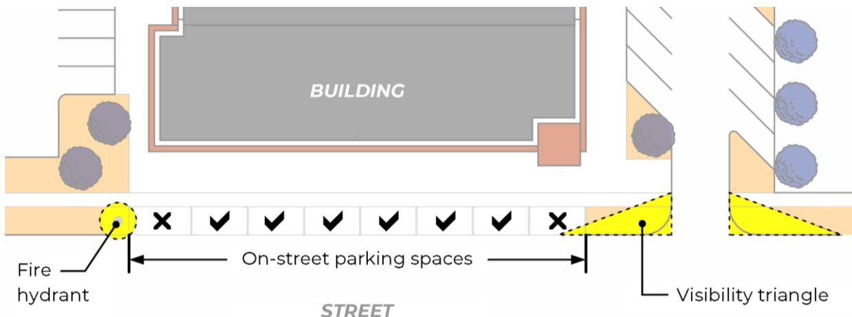
Figure 07.07-1: Visibility Triangle Limitations to On-Street Spaces
