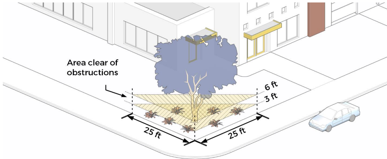
Figure 03.05-2: Visibility Triangle at Intersections
