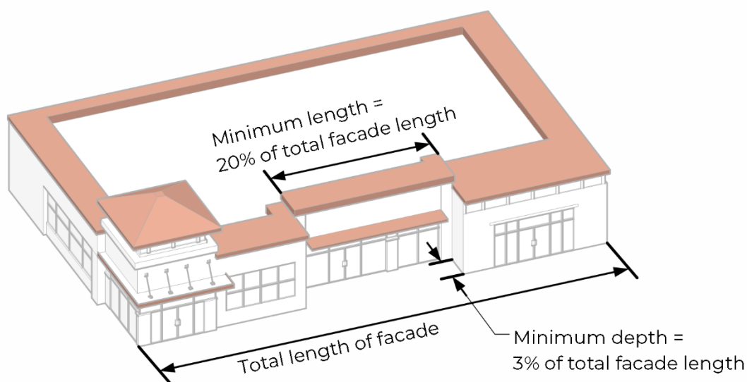
Figure 07.11-1: Wall Plane Articulation Requirement
