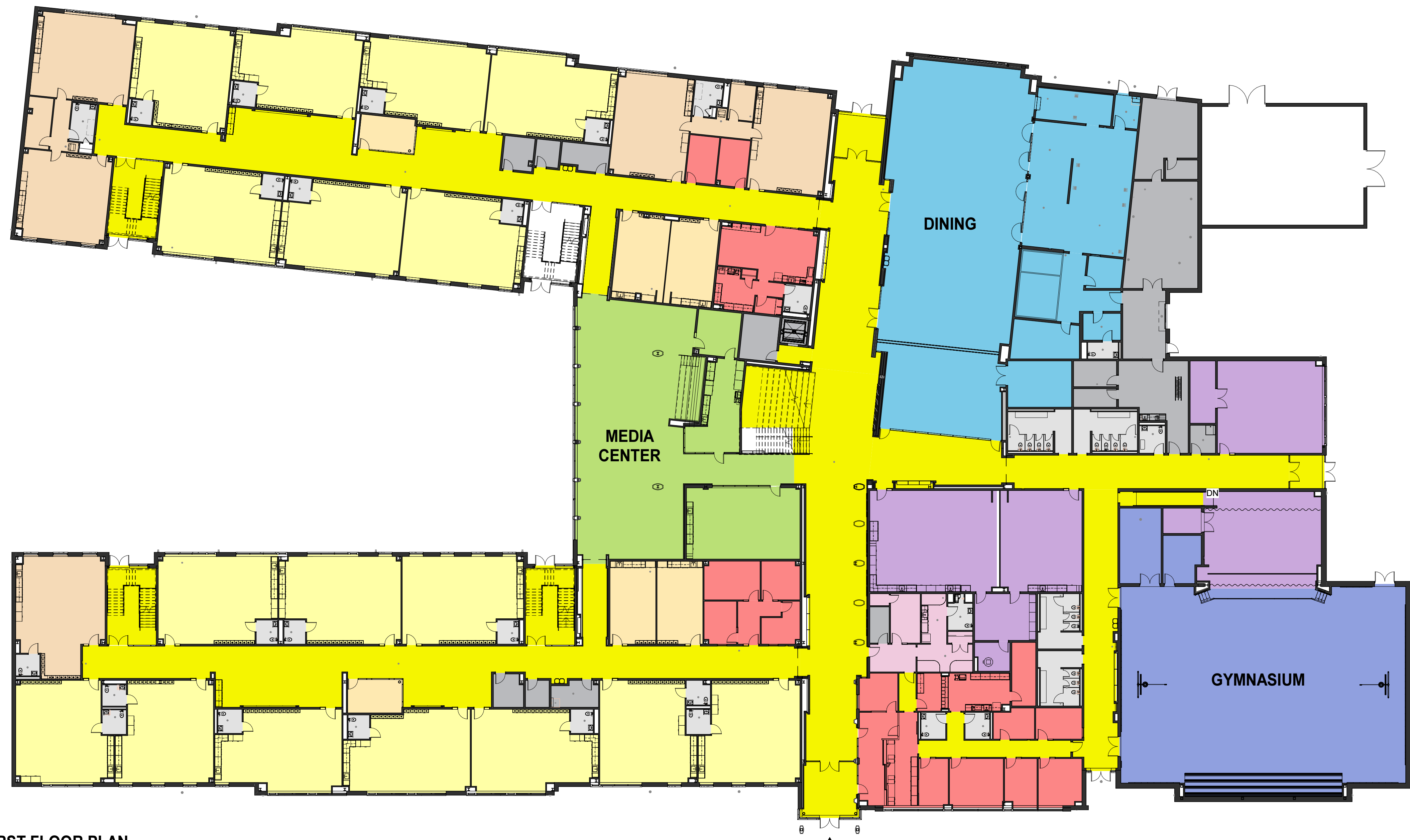
FIRST FLOOR PLAN 1" = 20'-0"
