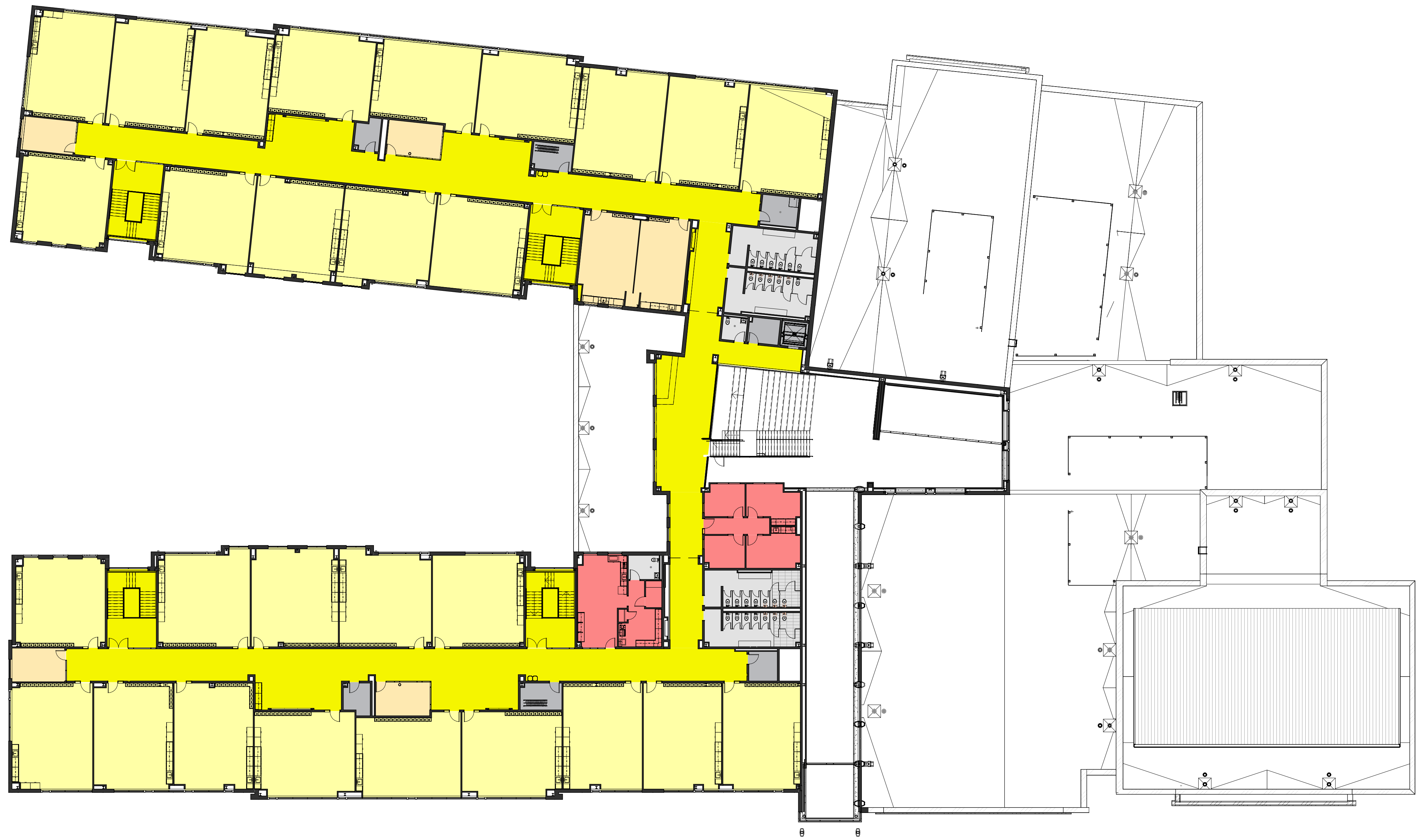
SECOND FLOOR PLAN 1" = 20'-0"
