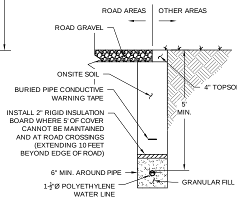
4 WATER LINE DETAIL NOT TO SCALE NOTE: WATER LINE TO BE DISINFECTED AND TESTED WITH LOCAL PUBLIC WORKS DEPARTMENT REQUIREMENTS
