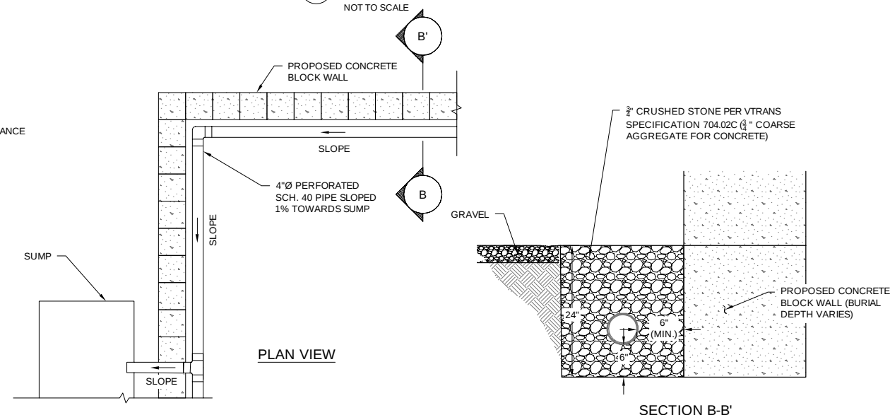
7 PERIMETER DRAIN DETAIL
