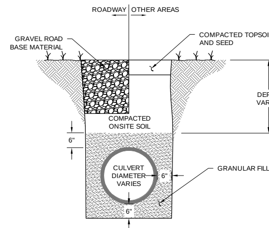
2 TYPICAL CULVERT DETAIL
