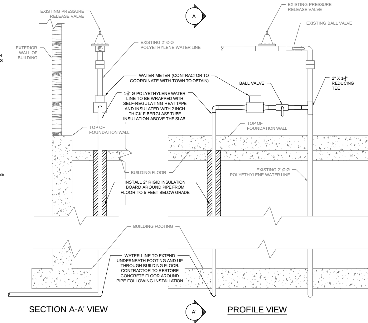
5 WATER LINE CONNECTION DETAIL
