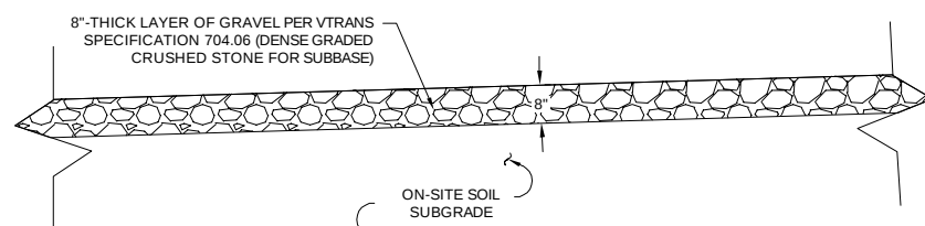
6 TYPICAL GRAVEL DETAIL NOT TO SCALE
