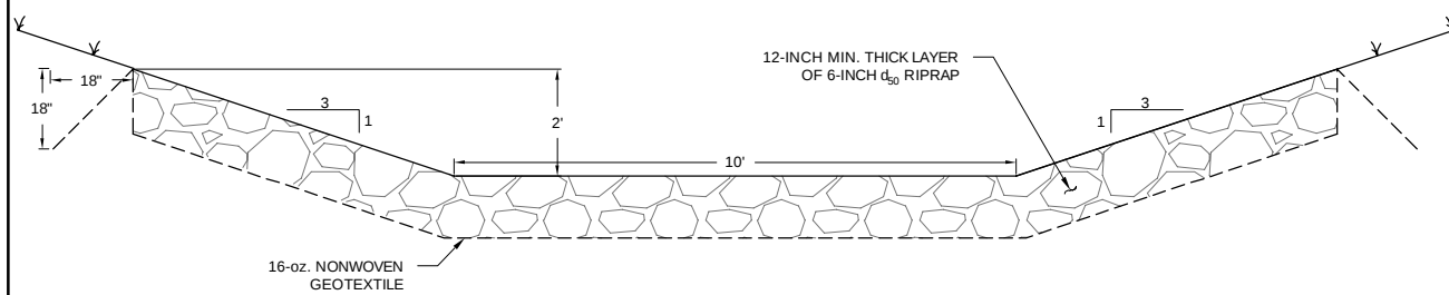
RIPRAP SPILLWAY DETAIL
