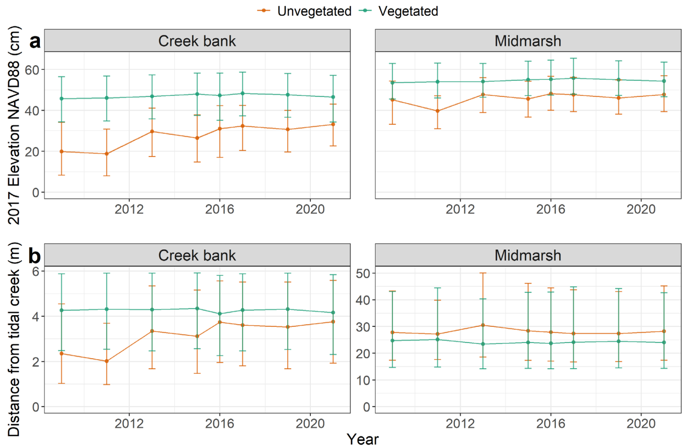
FIGURE 3 Characterization of unvegetated and vegetated areas within the West Ashley, SC, salt marsh. (a) Median \pm interquartile range of the field-corrected 2017 light detection and ranging derived digital elevation model of vegetated and unvegetated areas over time. (b) Median \pm interquartile range of the distance from the closest tidal creek of vegetated and unvegetated areas over time. NAVD88, North American Vertical Datum of 1988.
