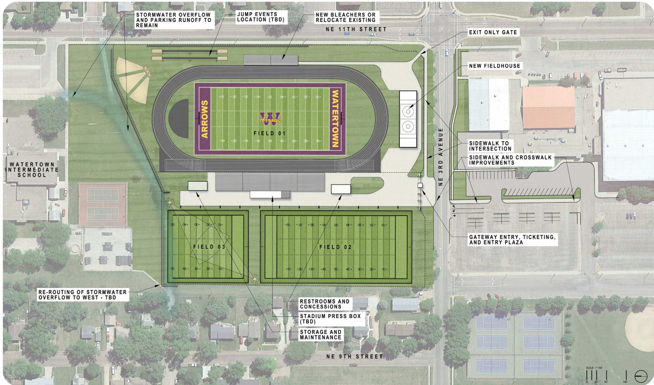
Site Concept Plan - Option 2 (Track Shifted North 80'-100') FUTURE PHASE WATERTOWN HIGH SCHOOL TRACK AND FIELD PLANNING
