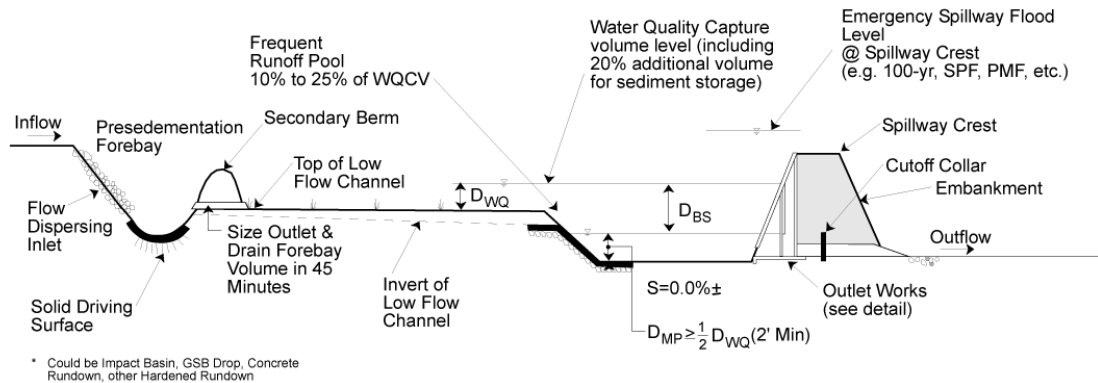
SECTION NOT TO SCALE
