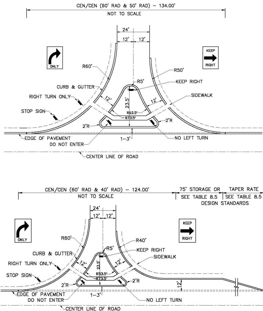
Figure 5.4: Right-In, Right-Out Driveway Designs
