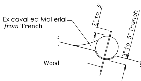
DETAIL 8 TYPICAL OF ALL INSTALLATIONS
