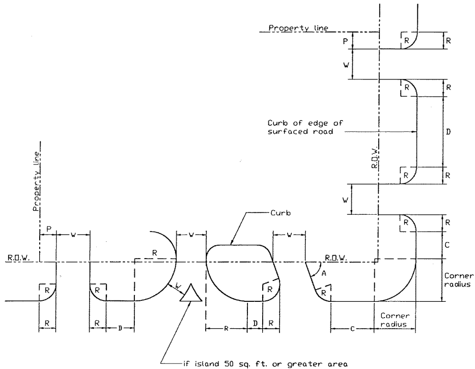
Figure 5.1 Driveway Dimensions
