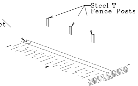
4 BACKFILL TRENCH AND WHEEL COMPACT SOIL
