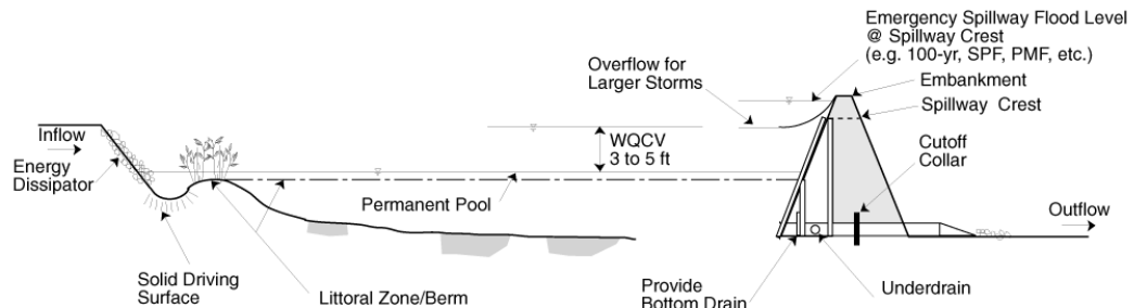
SECTION NOT TO SCALE
