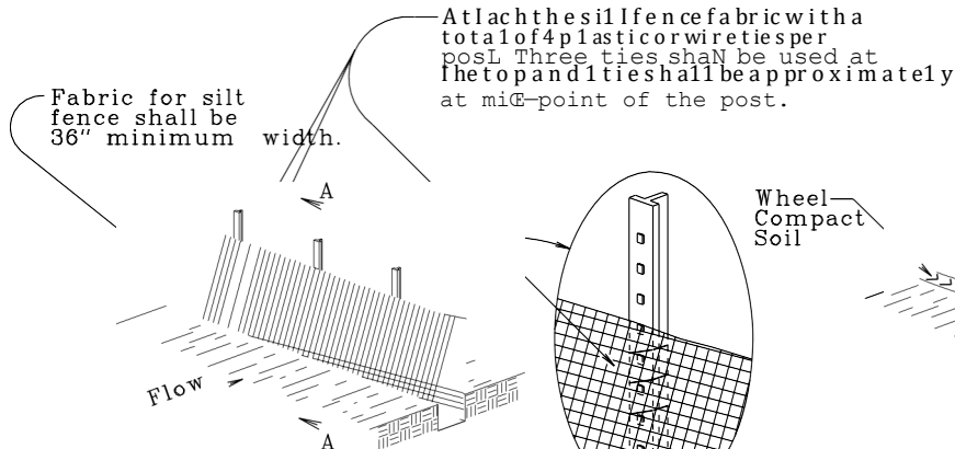
3 ATTACH SILT FENCE FABRIC
