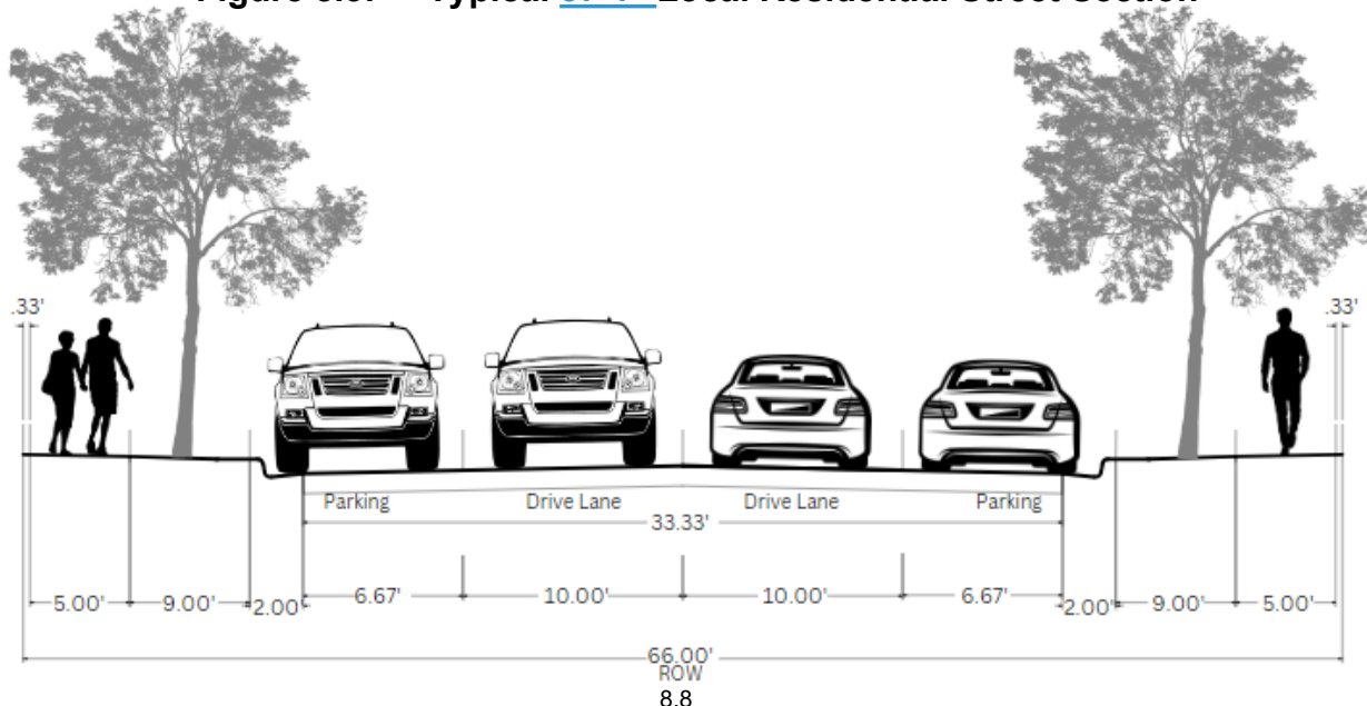
Figure 8.3: Typical 37'4" Local Residential Street Section
