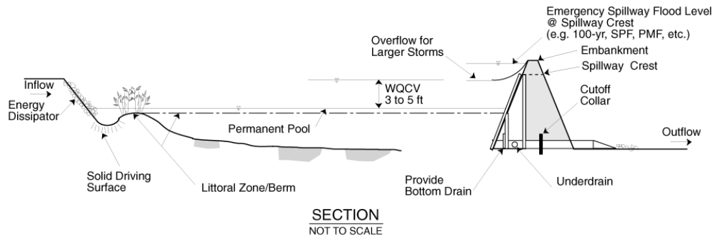
FIGURE RP-1 Plan and Section of a Wet Extended Detention Basin
