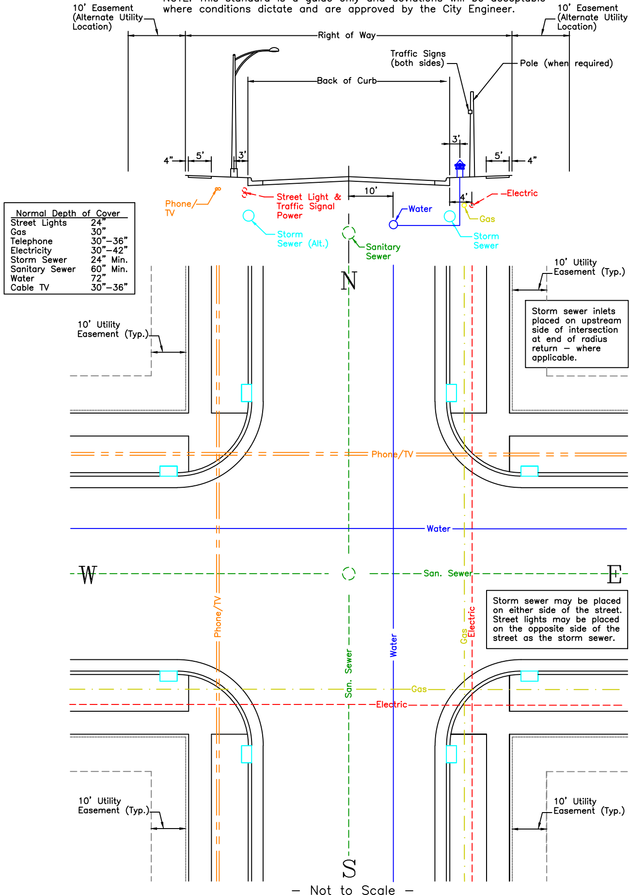
Figure 4.1 Standard Utility Locations
