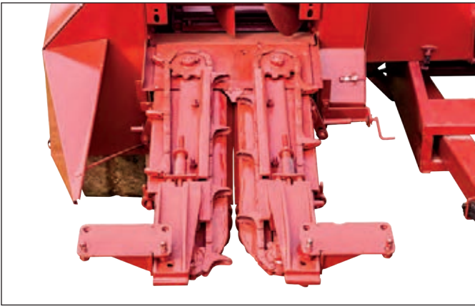
Combine corn head with deck plates and aggressive knife rolls
