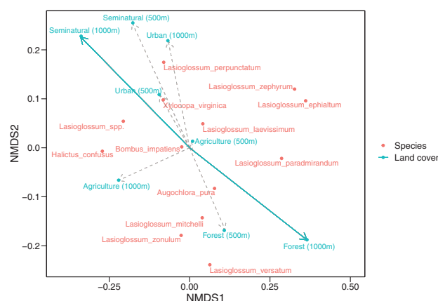
Fig. 4. Ordination plot showing the position of hemp visiting species (points) relative to the vectors of environmental variables (lines). Solid lines indicate that the environmental variable was significantly associated with variation in the community.
