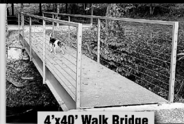
4'x40' Walk Bridge
