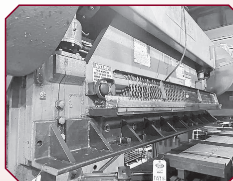
Cyril Bath Model C Press Brake Heavy duty industrial Mechanical Press Brake. 150 Ton Capacity with a 10' Bed Great for precision Sheet Metal Bending of stainless steel, mild steel, and aluminum parts. Price: $11,999.99
