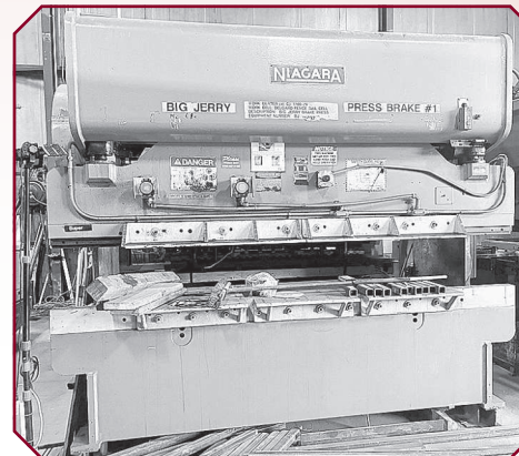
Niagara 60 Ton Press Brake Model 60-8-10 Mechanical Press Brake 10' Bed Total Bed Length Will Bend: 14Ga at 10', 12Ga at 8', 10Ga at 5' Price: $8,000
