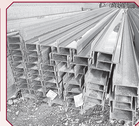
W6x12 I-Beam 6"Hx4"W (12 lbs per Foot) 24' Long (6 ea available) 20' Long (35 ea Available) Priced by the Pound: $0.65 per Pound (Approx: $7.80 per Foot)
