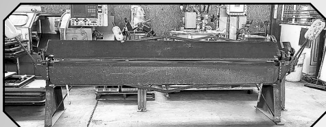
Chicago Dreis Break , Chicago Dreis & Krump MFG Model # S-1018, Up To 18 Gauge Capacity, Bending Length 10' $3,200
