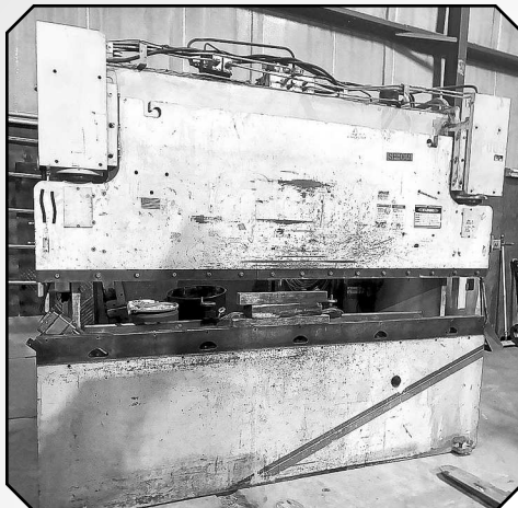
Wysong Hydraulic Press Brake , Wysong Press Brake 100 Ton, Model # MTH100-120, Stoke 8, Adjustment 9, does have a back gauge, $20,500
