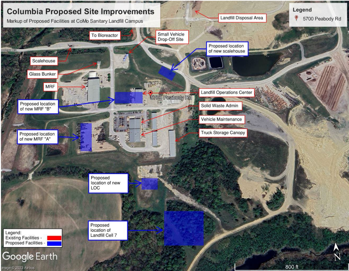
Figure 16: Aerial Photo of Columbia Landfill Property, Showing Proposed Locations for Infrastructure
