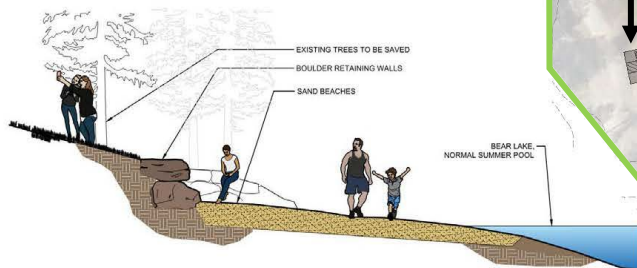
(A-A) CONCEPTUAL BEACH SECTION 1/4\"/>
