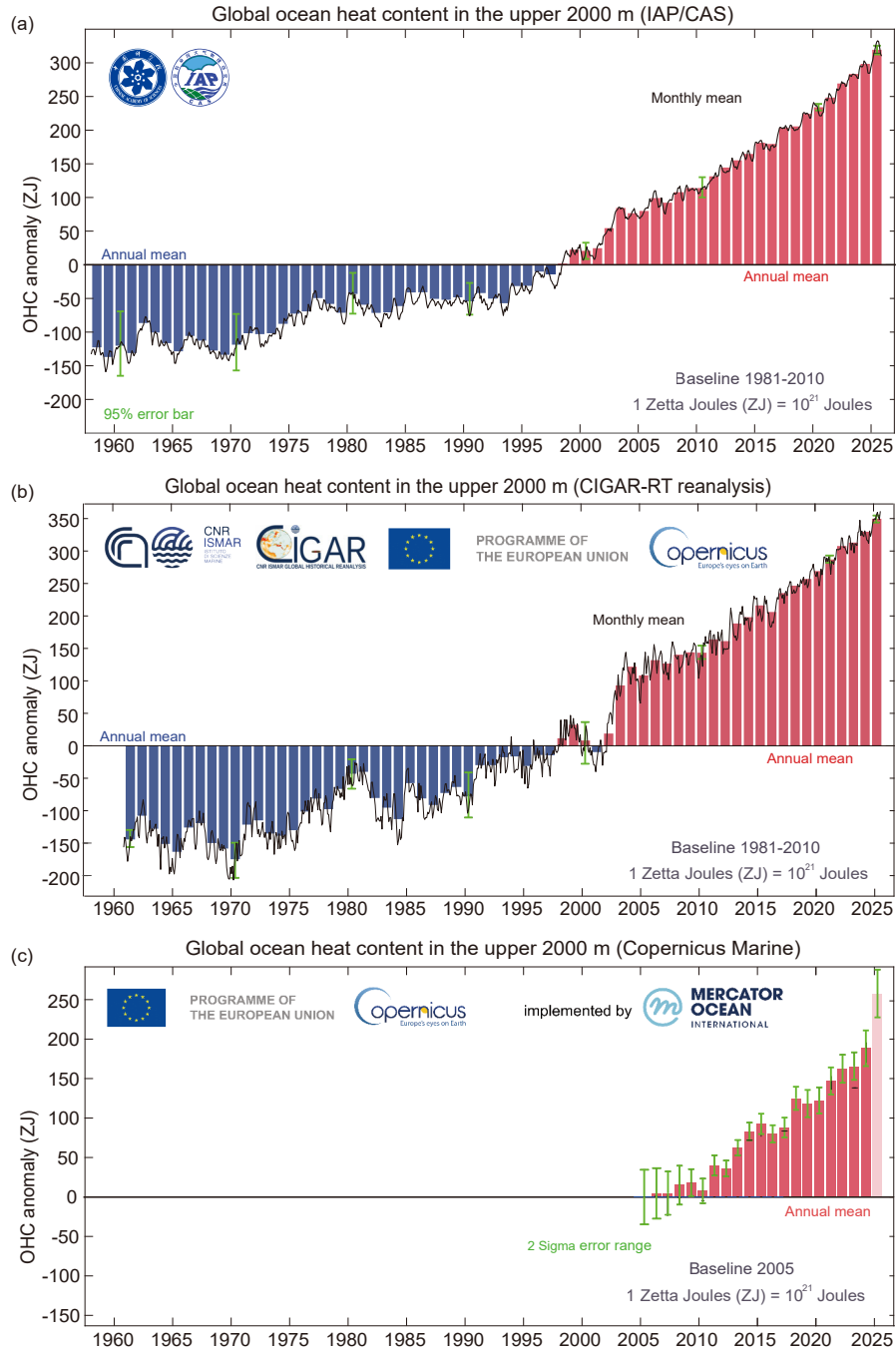
Fig. 1. Global upper 2000 m OHC from 1958 through 2025 according to (a) IAP/CAS, (b) CIGAR-RT (from 1961 through 2025), and (c) Copernicus Marine (from 2005 through 2025) ( 1 \text{ ZJ} = 10^{21} \text{ J} ). In panels (a) and (b), the black curves represent monthly time series, while the histograms show annual anomalies. In panel (c), 2025 data are preliminary (near real-time), plotted separately (light pink), and might be not fully representative. All time series are referenced to the 1981–2010 climatology for the IAP/CAS and CIGAR-RT products, and to a 2005 reference level for the Copernicus Marine product. For reference, the 2005 OHC values relative to the 1981–2010 baseline are 78 ZJ for IAP/CAS and 104 ZJ for CIGAR-RT. Uncertainty estimates from the different datasets are illustrated by the green bars. Note that the y-axis scales differ among panels.
