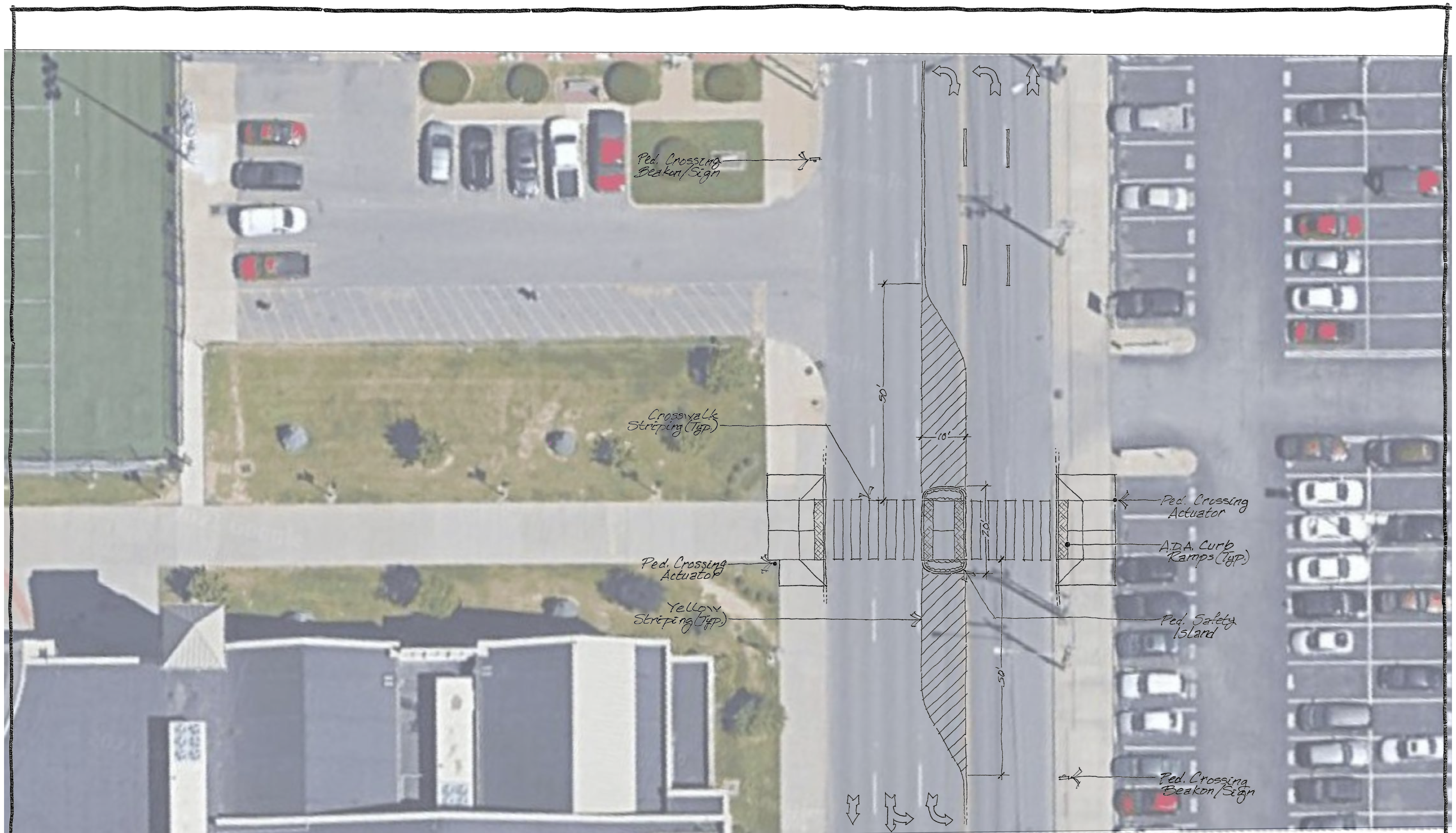
20th Street Pedestrian Crossing - Concept 2 City of Huntington, West Virginia Scale: 1" = 10'
