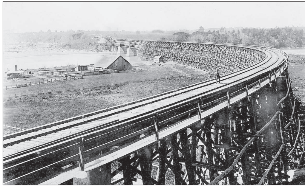
This view of the train trestle over the Chetco River, looking north, dwarfs a worker walking on the tracks. To the left is the McVay Ranch. Photo courtesy the McVay Collection and Chetco Valley Historical Society Museum.
