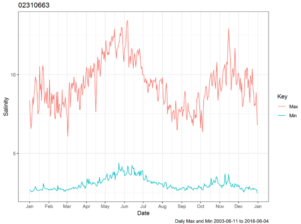
Figure 2-24. Salinity on day of year at Chassahowitzka River near Chassahowitzka, FL gage (No. 02310663).
