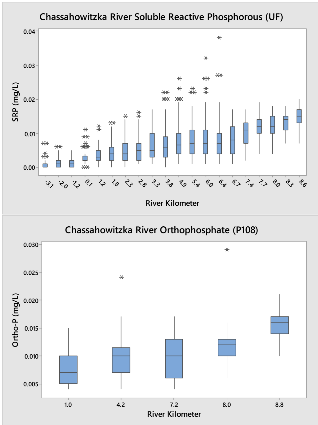
Figure 3-13. Distribution of soluble reactive phosphorous concentrations from the University of Florida 5 Rivers Project (UF) transect data collection effort between 1998 and 2011, and the Coastal Rivers Project (P108) active water quality sampling network between 2006 and 2017.
