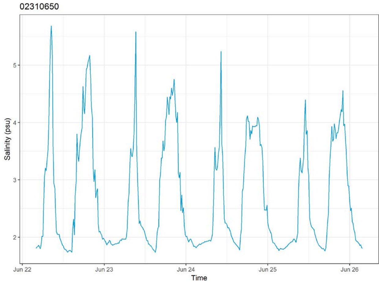
Figure 2-17. Tidal change in salinity at Chassahowitzka near Homosassa, FL gage (No. 02310650) June 22 to June 26, 2016.
