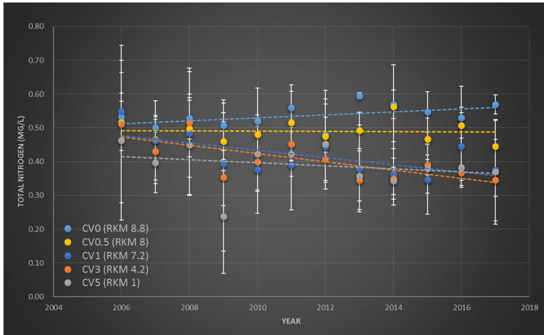
Figure 3-19. River-wide average annual total nitrogen across the period 2006 through 2017 for the five Coastal Rivers Project P108 fixed water quality monitoring stations.
