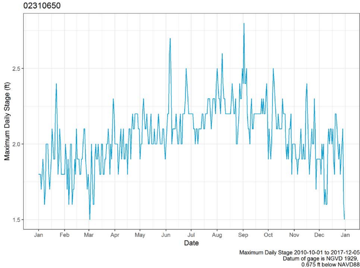
Figure 2-10. Average stage at day of year at Chassahowitzka River near Homosassa, FL gage (No. 02310650).
