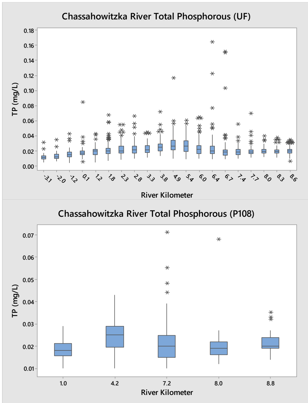
Figure 3-12. Distribution of total phosphorous concentrations from the University of Florida 5 Rivers Project (UF) transect data collection effort between 1998 and 2011, and the Coastal Rivers Project (P108) active water quality sampling network between 2006 and 2017.
