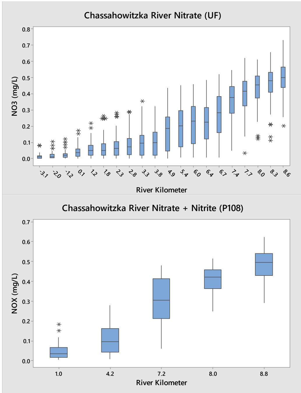
Figure 3-10. Distribution of nitrate concentrations from the University of Florida 5 Rivers Project (UF) transect data collection effort between 1998 and 2011, and the Coastal Rivers Project (P108) active water quality sampling network between 2006 and 2017.
