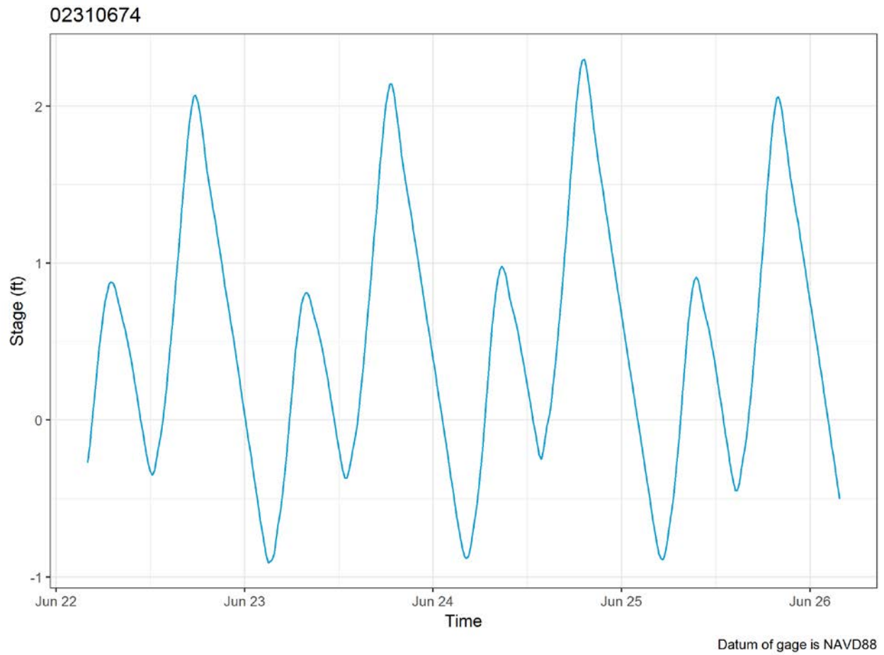
Figure 2-31. Tidal cycle in stage at Chassahowitzka River at Mouth near Chassahowitzka, FL gage (No. 02310674).
