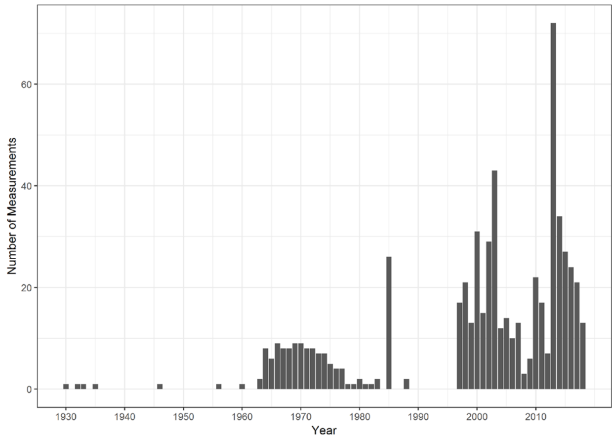
Figure 2-14. History of field measurements of flow at Chassahowitzka near Homosassa, FL gage (No. 02310650).
