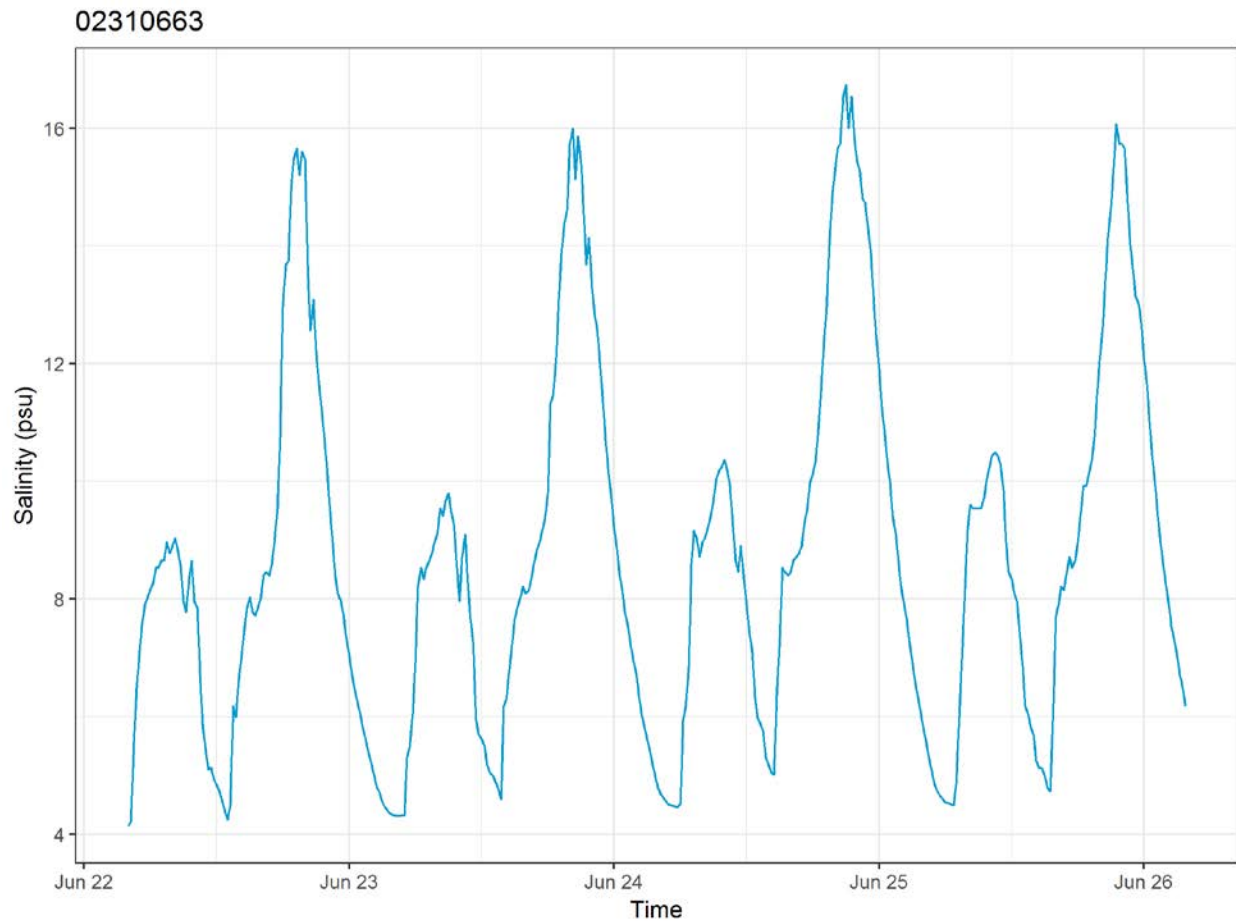
Figure 2-23. Tidal cycles in salinity at Chassahowitzka River near Chassahowitzka, FL gage (No. 02310663) from June 22 to June 26, 2017.
