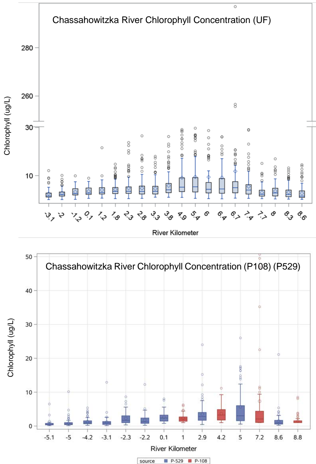
Figure 3-15. Distribtuon of chlorophyll concentrations from the University of Florida 5 Rivers Project (UF) transect data collection effort between 1998 and 2011 and at fixed locations in the Chassahowitzka River from the Coastal Rivers Project (P108) and COAST Project (P529) active sampling networks in the Chassahowitzka River. Note broken y-axis for UF data in top panel.
