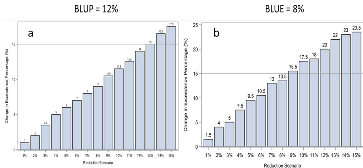
Figure 3-32. Critical flow reductions corresponding to 15% increased relative risk of exceedance of a 3.9 µg/L chlorophyll NNC threshold as predicted by BLUPs (a) and BLUEs (b). Relative risks are compared between flow reduction scenarios and the unimpacted flow scenario. Horizontal line corresponds to 15% increased relative risk. Numbers above bars represent the relative risk compared to unimpacted for each flow reduction scenario. Reproduced from Janicki Environmental, Inc. (2018) figure 4-3.
