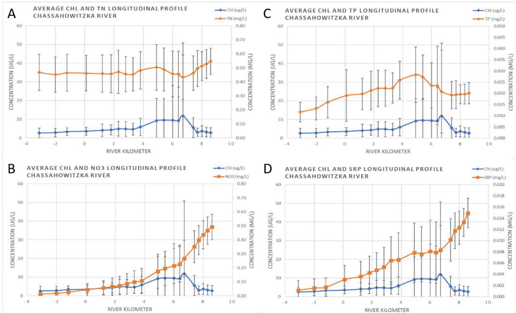
Figure 3-16. Relationship between chlorophyll concentration and various nutrient concentrations from the University of Florida 5 River Project transect data collection effort between 1998 and 2011. Panels represent chlorophyll and total nitrogen (A), chlorophyll and nitrate (B), chlorophyll and total phosphorous (C), and chlorophyll and soluble reactive phosphorous (D), respectively.
