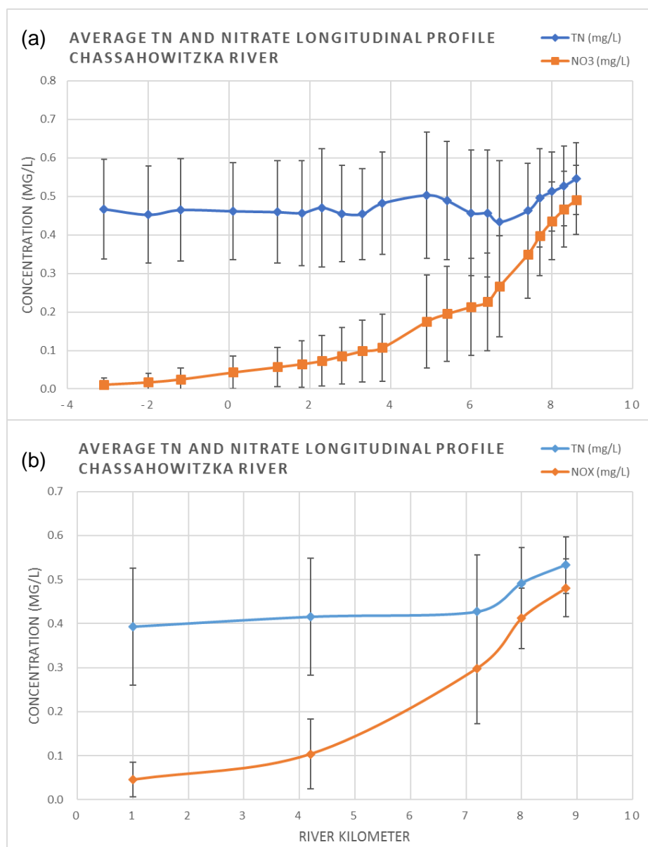
Figure 3-11. Longitudinal profiles of total nitrogen and nitrate concentrations from (a) the University of Florida 5 Rivers Project transect data collection effort between 1998 and 2011, and (b) the Coastal Rivers Project P108 active water quality sampling network between 2006 and 2017.
