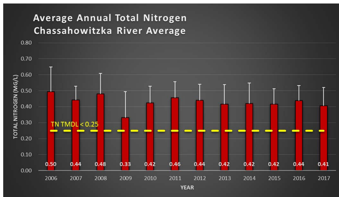
Figure 3-18. River-wide average annual total nitrogen concentration for the period 2006 through 2017. Data are from the five P108 fixed stations. Yellow dashed line depicts the TN TMDL of 0.25 mg/L for the Chassahowitzka River WBID 1361.
