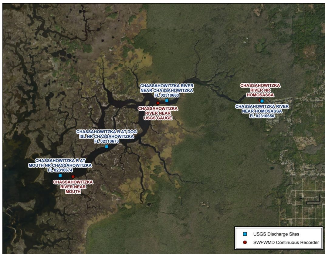
Figure 3-5. Location of the three District continuous recorders (red circles) for water quality on the Chassahowitzka River. Blue squares show the locations of the USGS river discharge gages. The most upstream USGS gage – Chassahowitzka River near Homosassa, FL (gage No. 02310650) – also has a continuous nitrate sensor.
