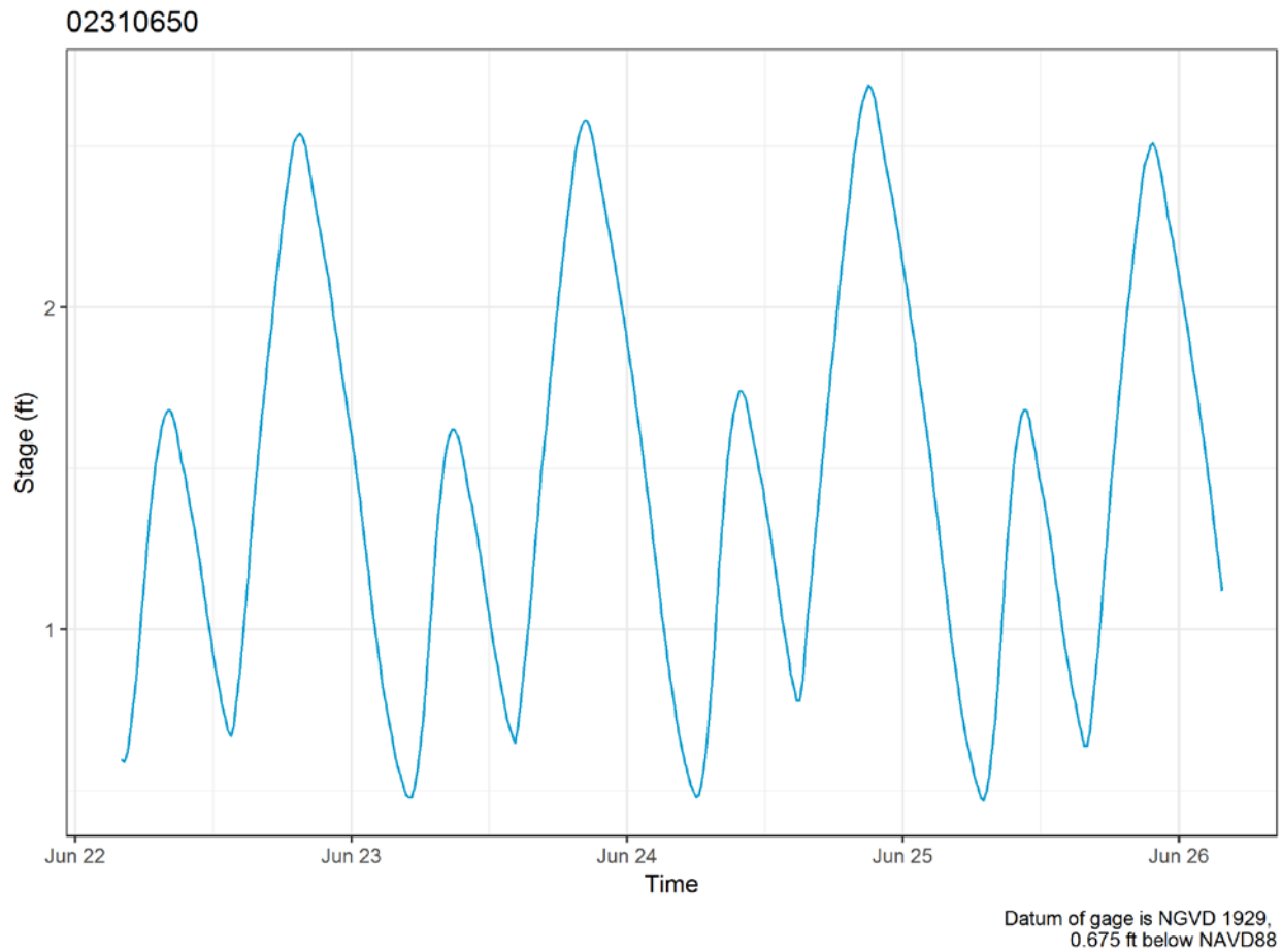
Figure 2-9. Tidal stage at Chassahowitzka River near Homosassa, FL gage (No. 02310650). Data shown from June 22 to June 26, 2016 to illustrate typical tidal cycles.
