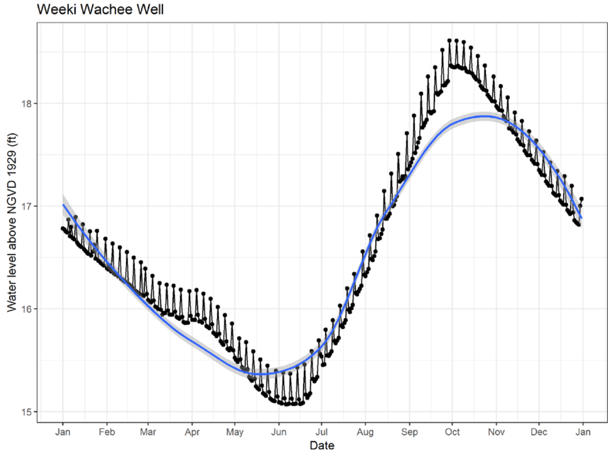
Figure 2-16. Average daily water levels in Weeki Wachee Well USGS 283201082315601 for day of year over long-term period of record (06/15/1966 to 12/11/2017). Blue lines are loess smoothers with grey standard error. Points show average values, and black lines are linear interpolation between data points. Spikes can be seen on 5, 10, 15, 20, 25, 30 of each month because measurements were only taken on those dates prior to 1974-10-01, skewing those particular days of the month to higher values. The well was relocated on 2013-04-30, which has been adjusted by adding 0.3 ft to match with old well location following regression adjustment by USGS (Kevin Grimsley, personal communication, 2018).
