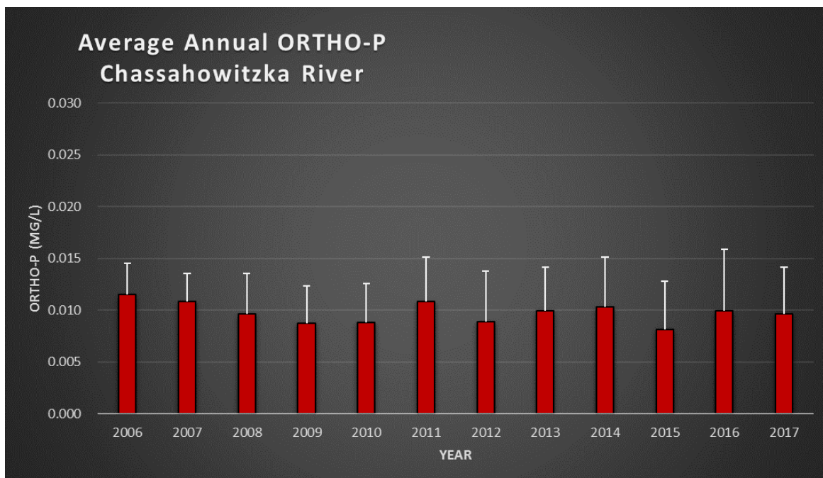
Figure 3-25. River-wide average orthophosphorous concentrations for the period 2006 through 2017. Data are from the five P108 fixed stations.
