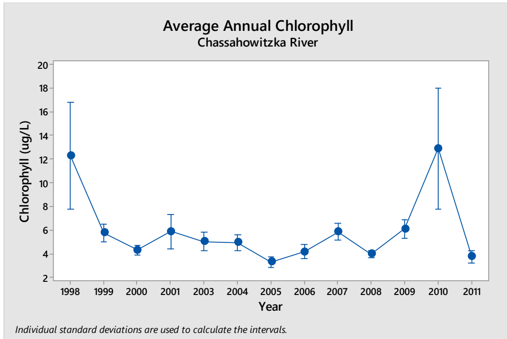
Figure 3-28. River-wide average chlorophyll concentrations for the period 1998 through 2011. Data are from the University of Florida 5 Rivers Project.
