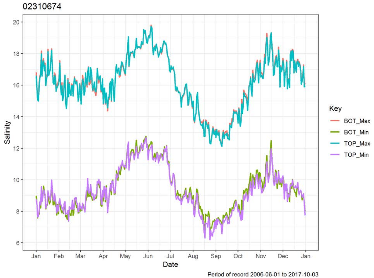
Figure 2-32. Daily minima and maxima in salinity at Chassahowitzka River at Mouth near Chassahowitzka, FL gage (No. 02310674).
