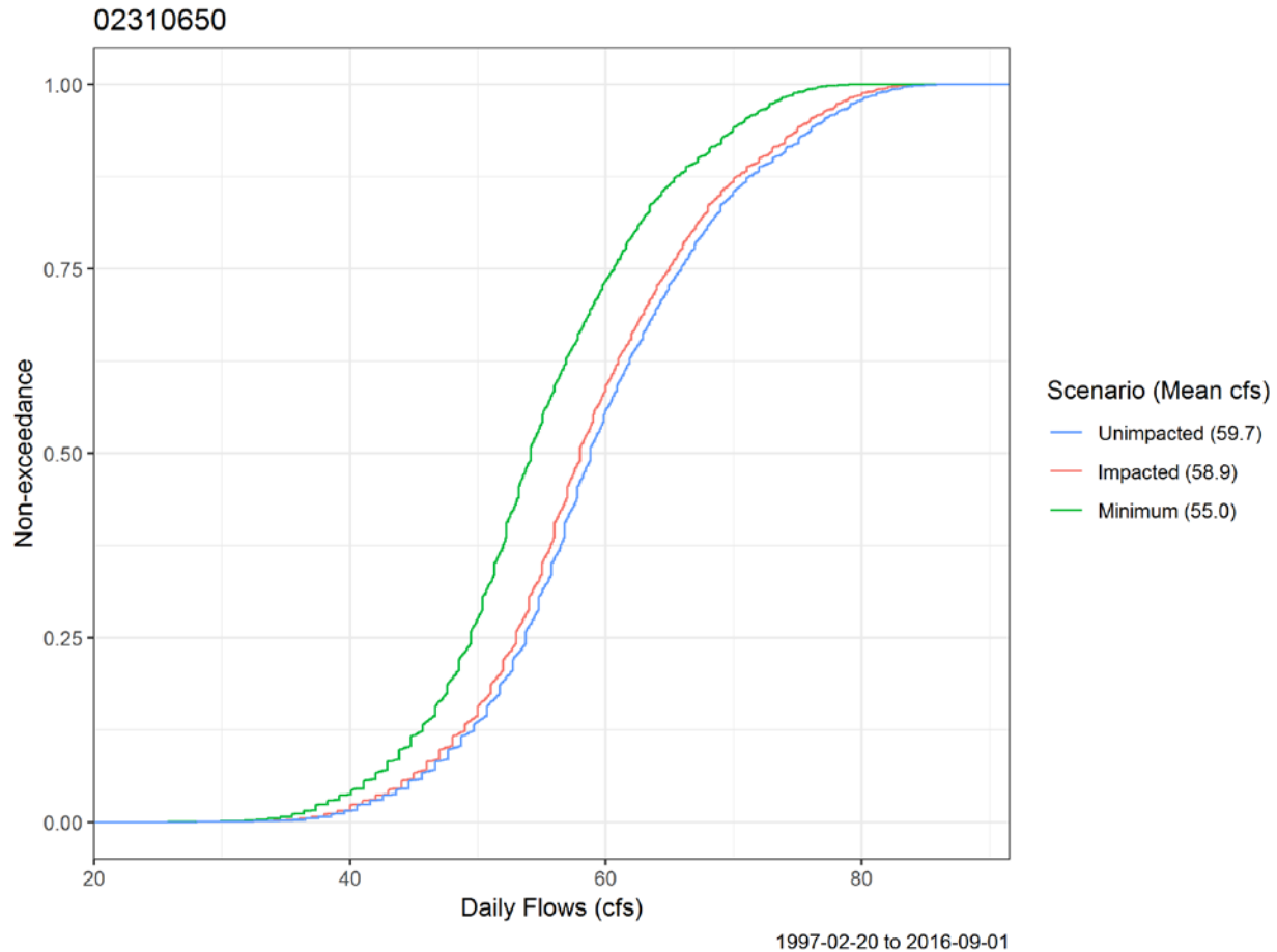
Figure 7-1. Daily flow scenarios for Chassahowitzka Main Spring gage 02310650.
