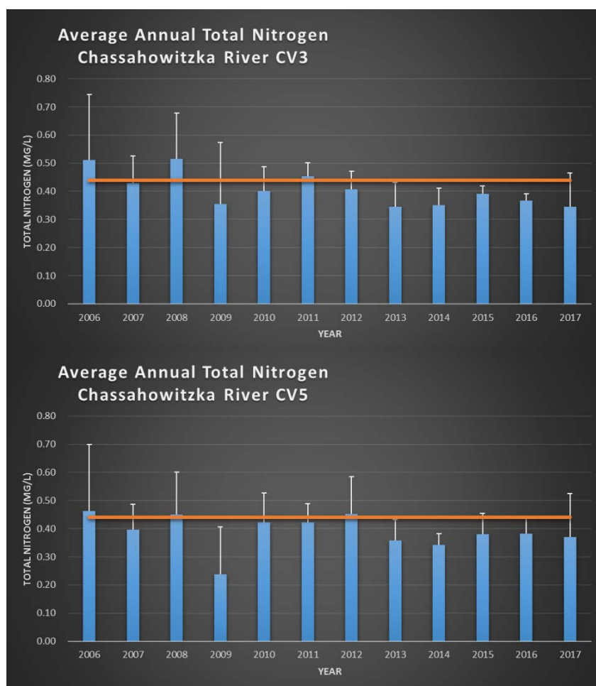
Figure 3-21. Total nitrogen time series from 2006 through 2017 for P108 stations CV3 (Rkm 4.2) and CV5 (Rkm 1). Orange reference lines represent the DEP site-specific NNC for the Chassahowitzka River estuary segment (WBID 1361).
