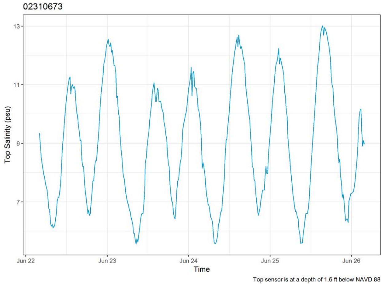
Figure 2-28. Tidal cycles in salinity at Chassahowitzka River at Dog Island near Chassahowitzka, FL gage (No. 02310673).
