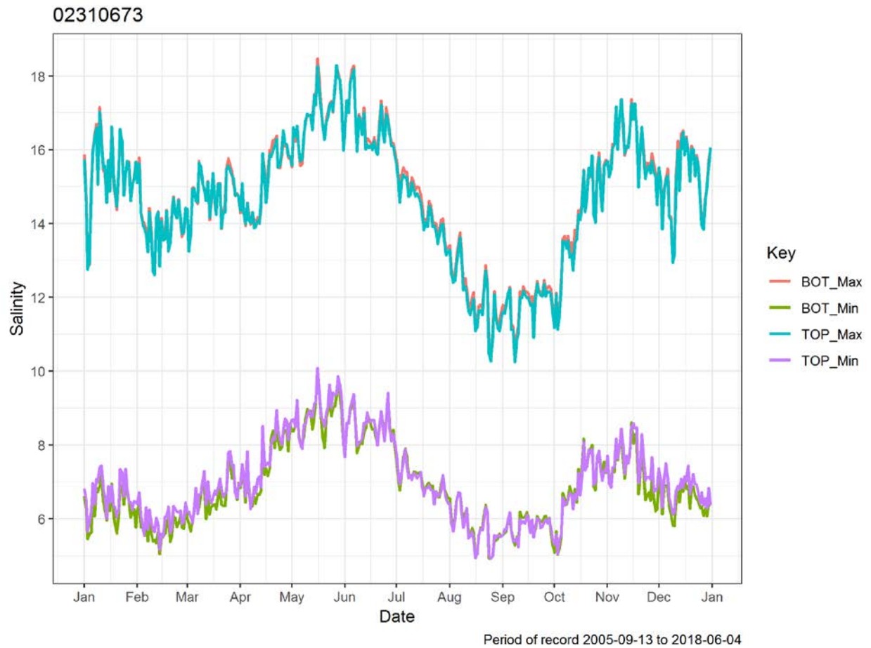
Figure 2-29. Daily minima and maxima in salinity at Chassahowitzka River at Dog Island near Chassahowitzka, FL gage (No. 02310673).
