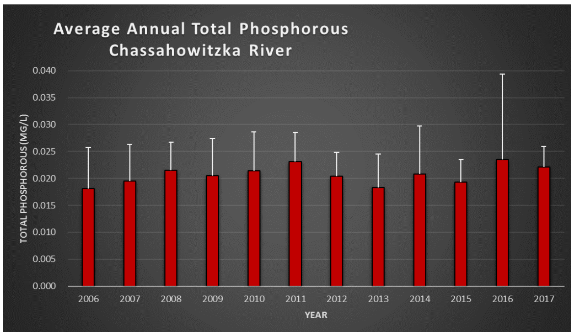
Figure 3-24. River-wide average total phosphorous concentrations for the period 2006 through 2017. Data are from the five P108 fixed stations.
