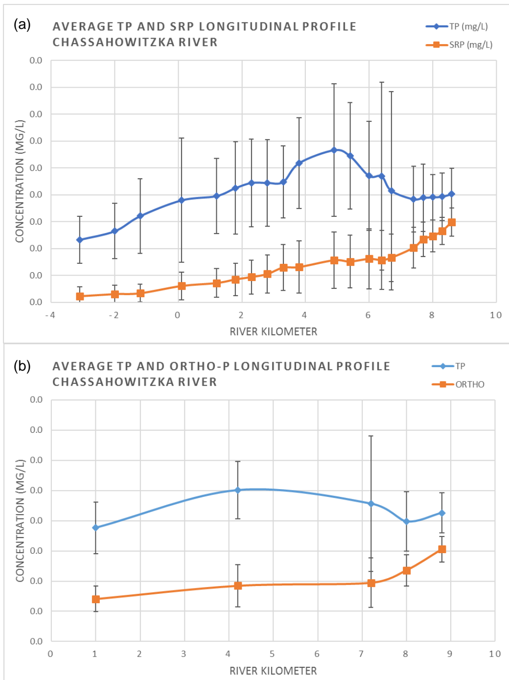
Figure 3-14 Longitudinal profiles of total phosphorous (TP) and soluble reactive phosphorous (SRP) concentrations from (a) the University of Florida 5 Rivers Project transect data collection effort between 1998 and 2011, and longitudinal profiles of total phosphorous (TP) and orthophosphorous (ORTHO) from the Coastal Rivers Project (P108) active water quality sampling network between 2006 and 2017.
