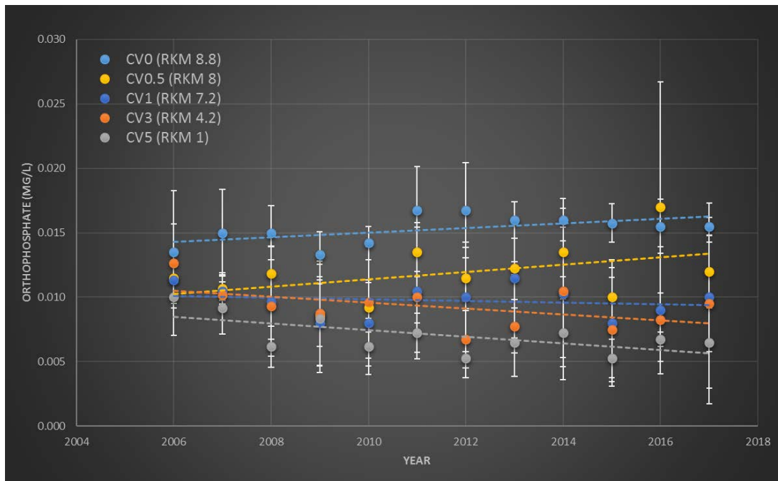
Figure 3-26. Average orthophosphate concentration by station for the period 2006-2017 for the five P108 fixed water quality monitoring stations.
