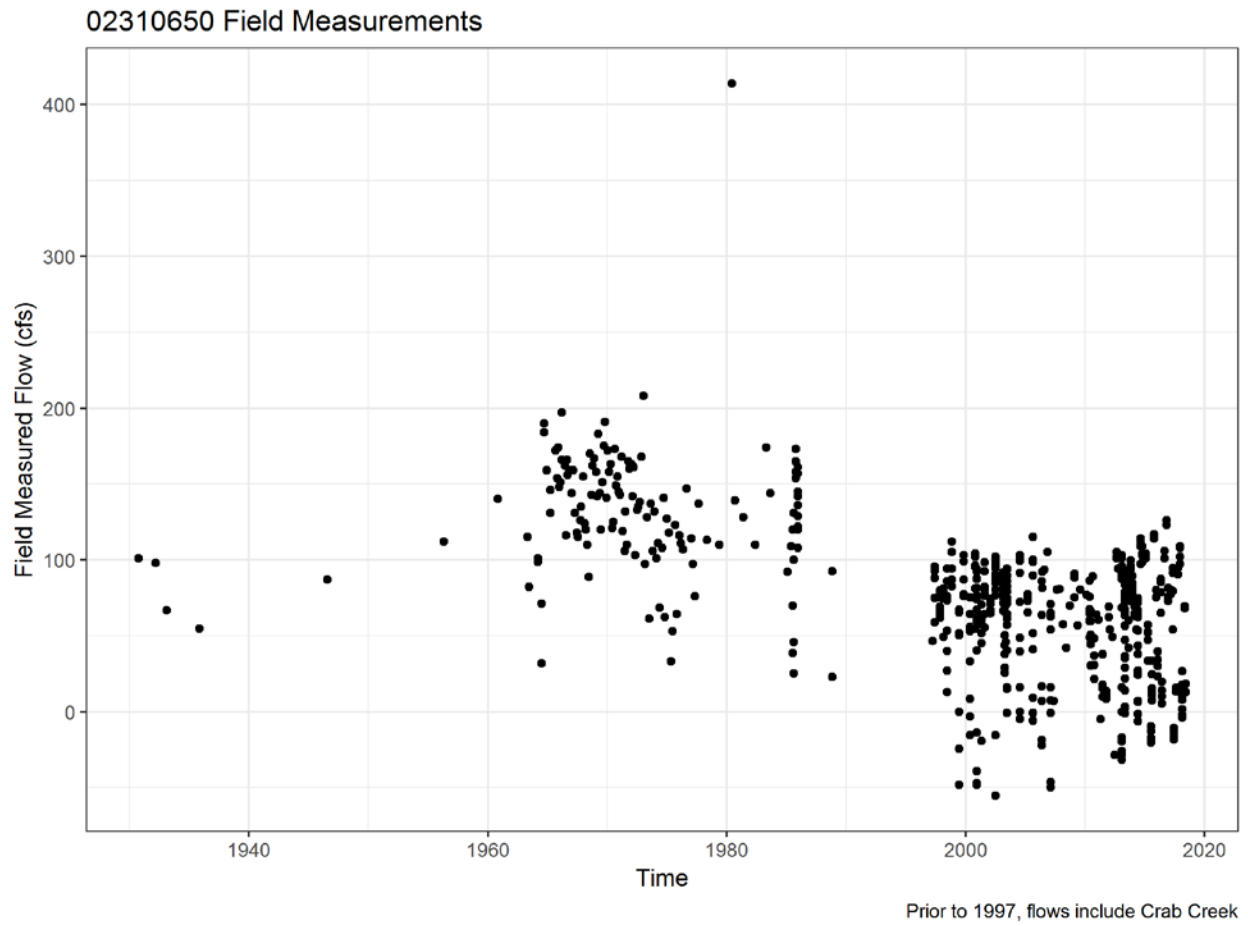
Figure 2-15. Field measurements of flow at Chassahowitzka near Homosassa, FL gage (No. 02310650). Prior to 1997, flows include Crab Creek (Heyl et al. 2012).
