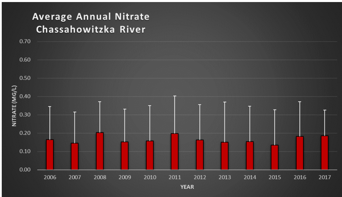
Figure 3-22. River-wide average annual nitrate concentration for the period 2006 through 2017. Data are from the five P108 fixed stations.
