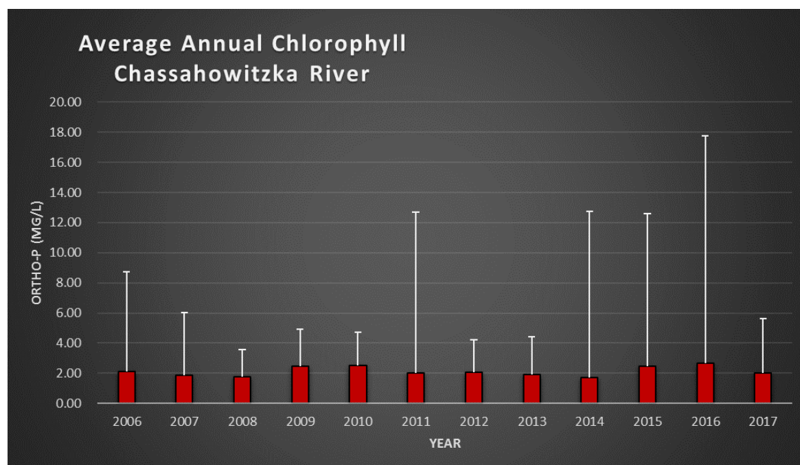
Figure 3-27. River-wide average chlorophyll concentrations for the period 2006 through 2017. Data are from the five Coastal Rivers Project P108 fixed stations.
