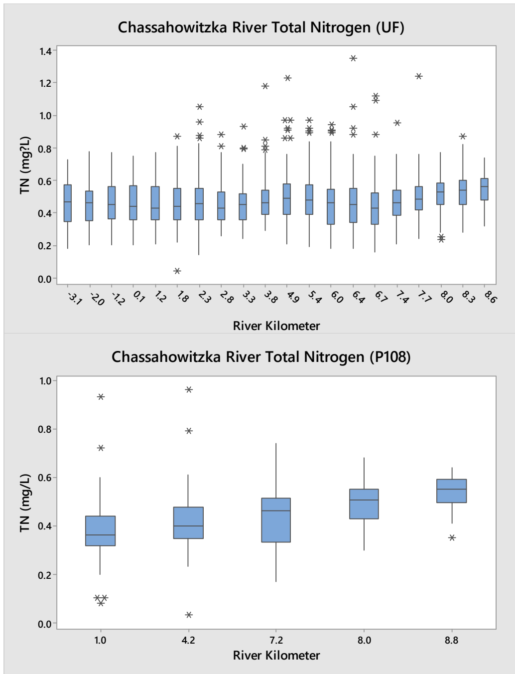
Figure 3-9. Distribtuon of total nitrogen concentrations from the University of Florida 5 Rivers Project (UF) transect data collection effort between 1998 and 2011 and from the active Coastal Rivers Project (P108) data collection effort between 2005 and 2017.
