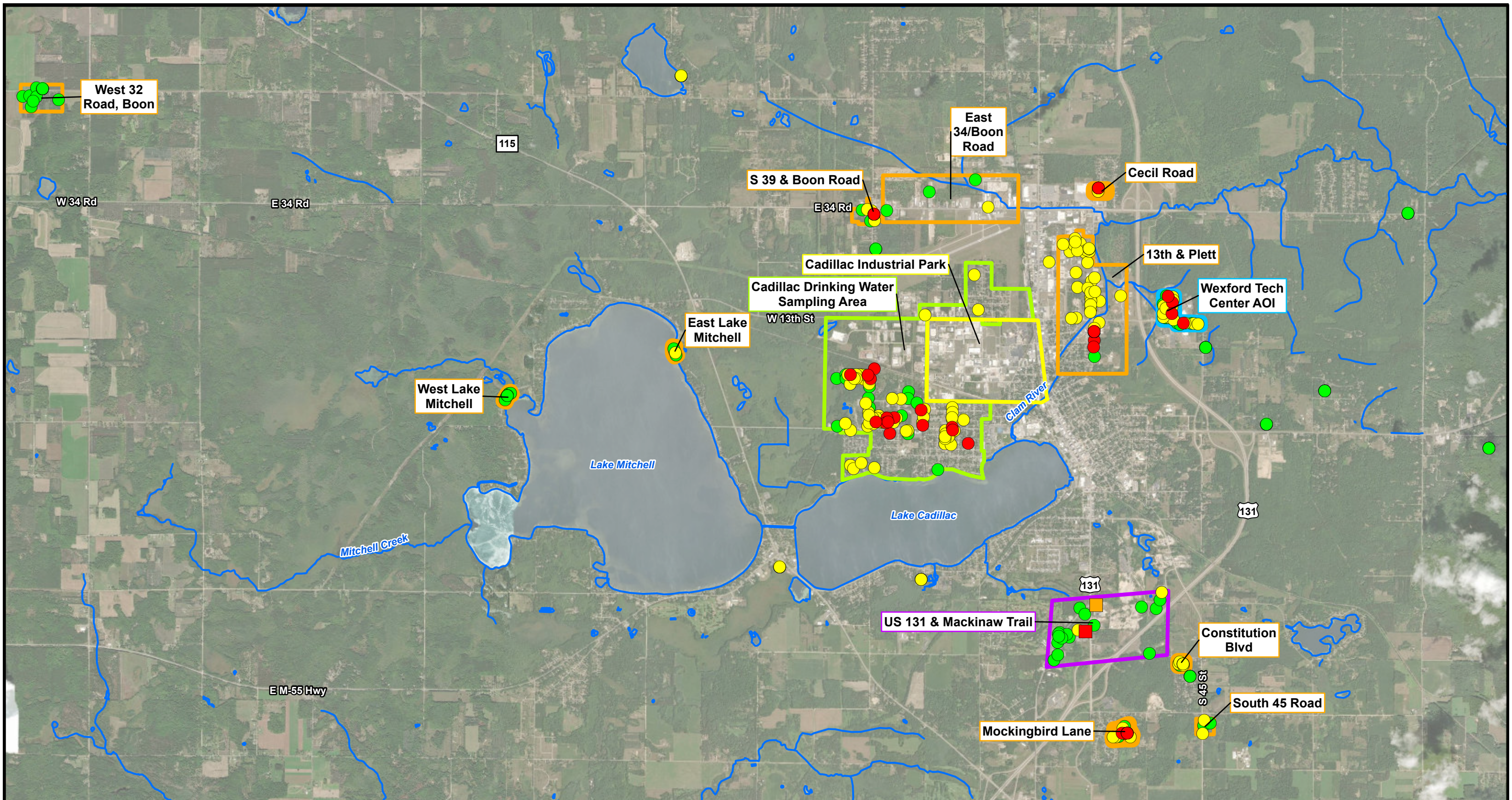
FIGURE 4 PFAS CRITERIA HEAT MAP
