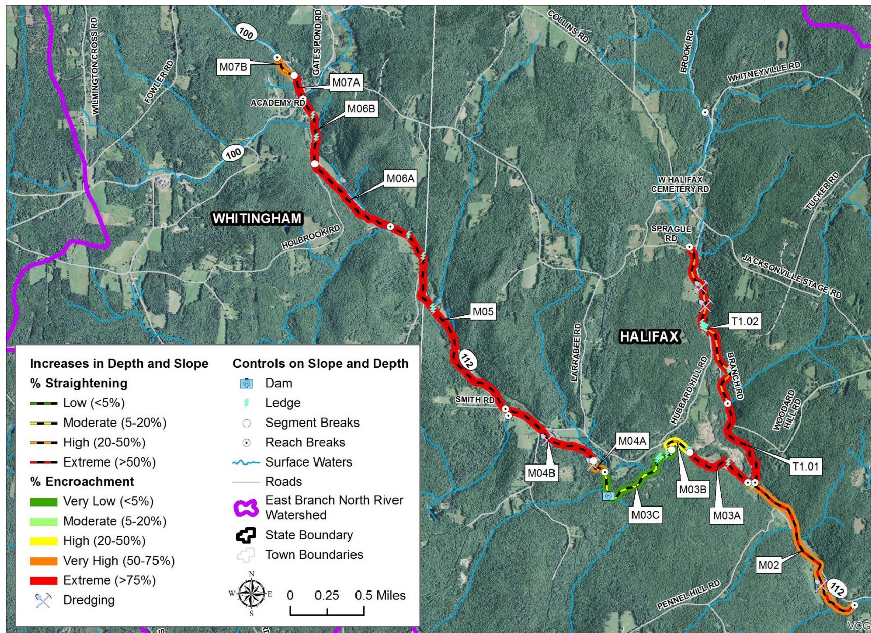
Figure 4.23: Controls on slope and depth for the East Branch North River watershed.
