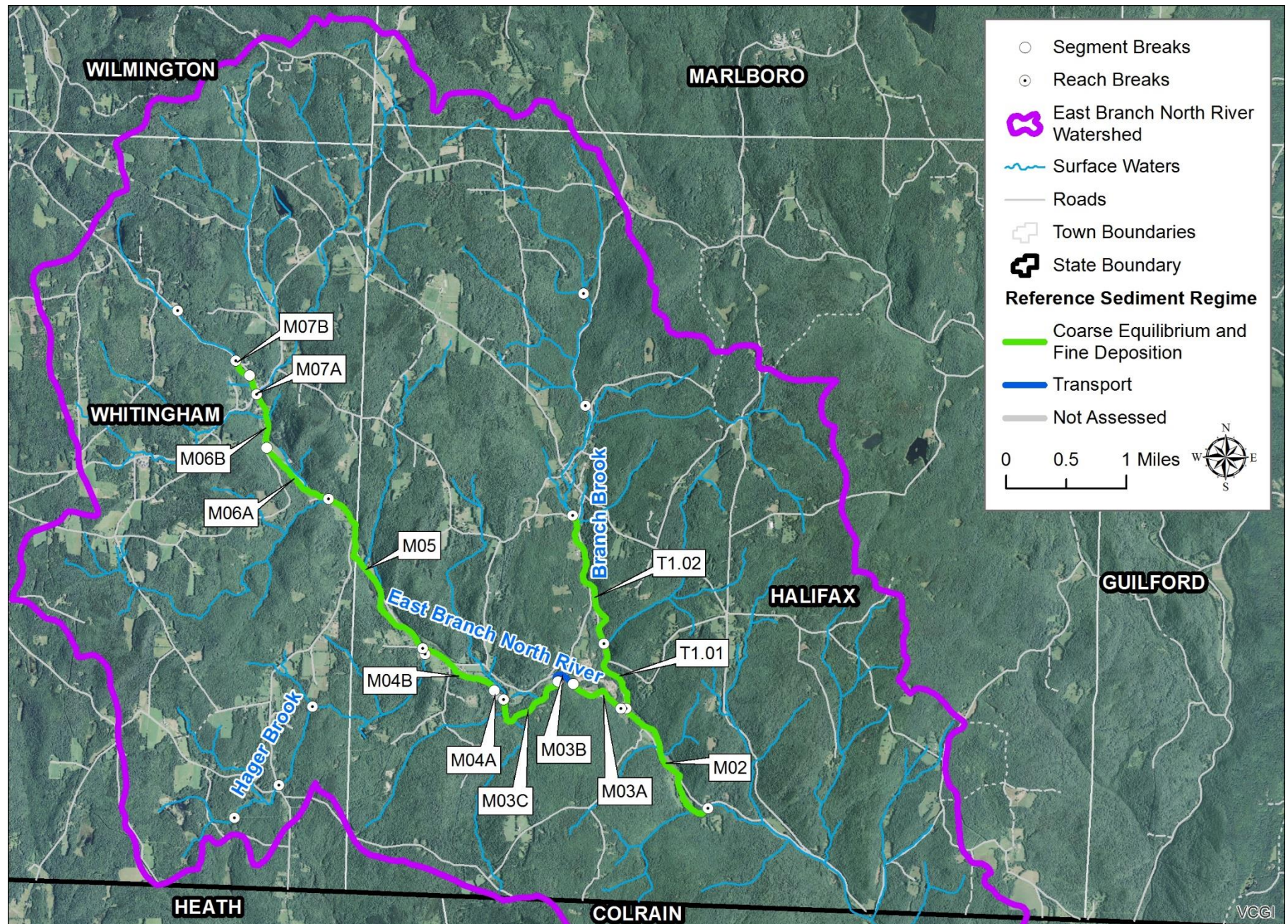
Figure 4.24: Reference Sediment Regime for the East Branch North River watershed.
